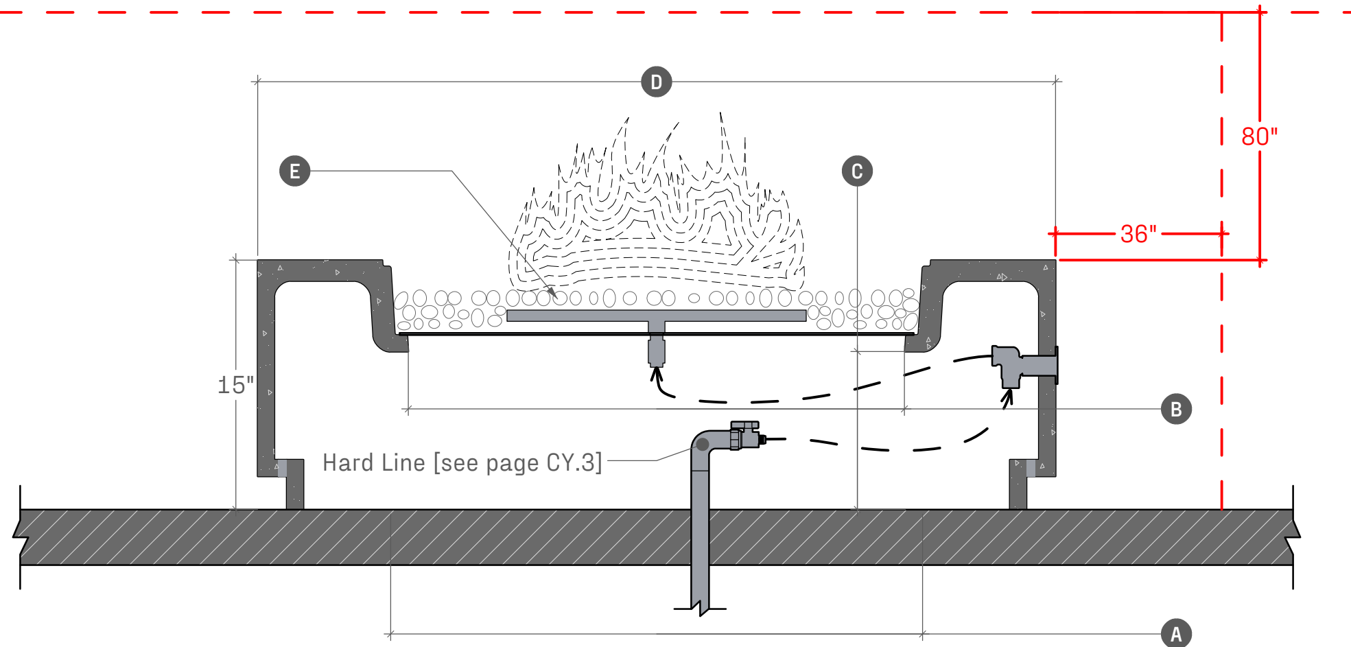
CY.2.1 SECTION DETAIL SCALE: 1" = 0' - 8"
