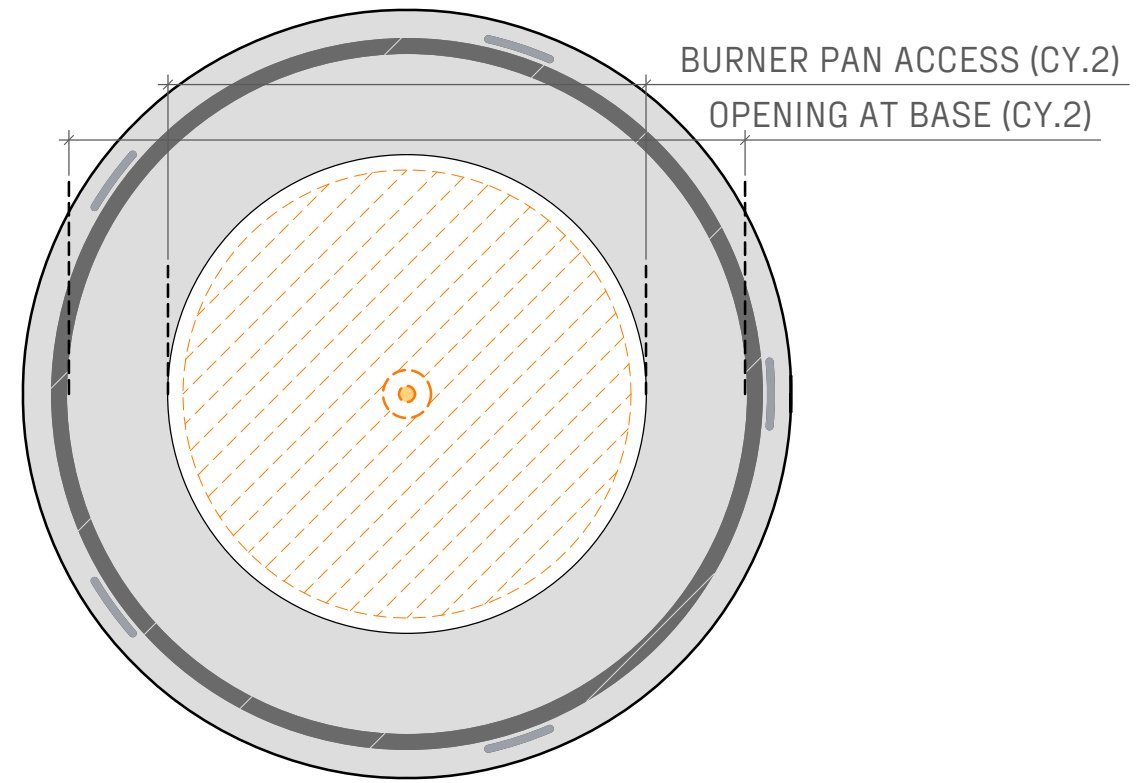
CY.3.2 PLAN VIEW SCALE: 1" = 1' - 0"
